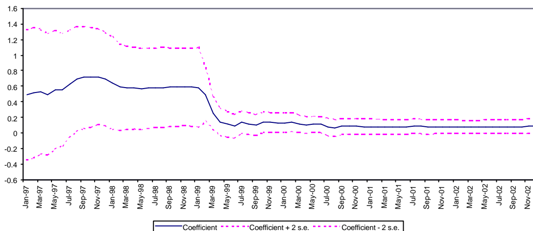
Figure 10 Recursive Estimates of the Coefficient on Exchange Rate Change
