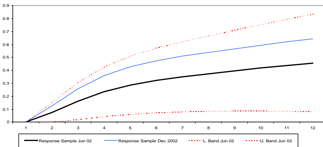
Figure 12 Impulse Responses of Price Level (IPCA) to an Exchange Rate Shock
