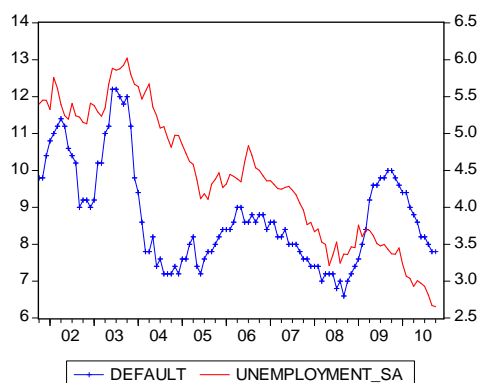
Figure 1: Default and unemployment rate, 2001:10 - 2010:10
