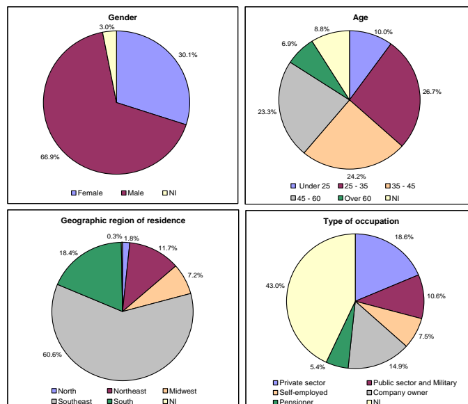
Figure 4: Descriptive Statistics – Vehicle Financing
