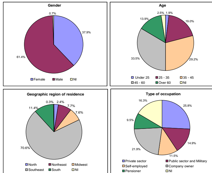
Figure 3: Descriptive Statistics – Consumer Credit
