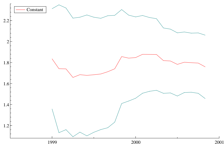
Figure 6: Recursive Estimation of the Intercept in Equation (6)
